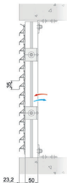
Corte DucoWall Classic W 20Z
